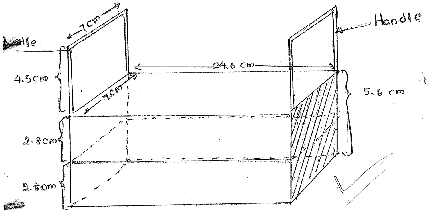
- Small size test tube rack with Handle -
