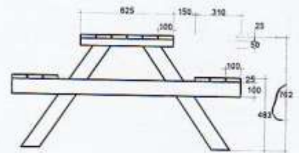
ELEVATION C
