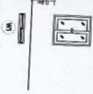
4' X 5' Aluminum framed double sash glass window
