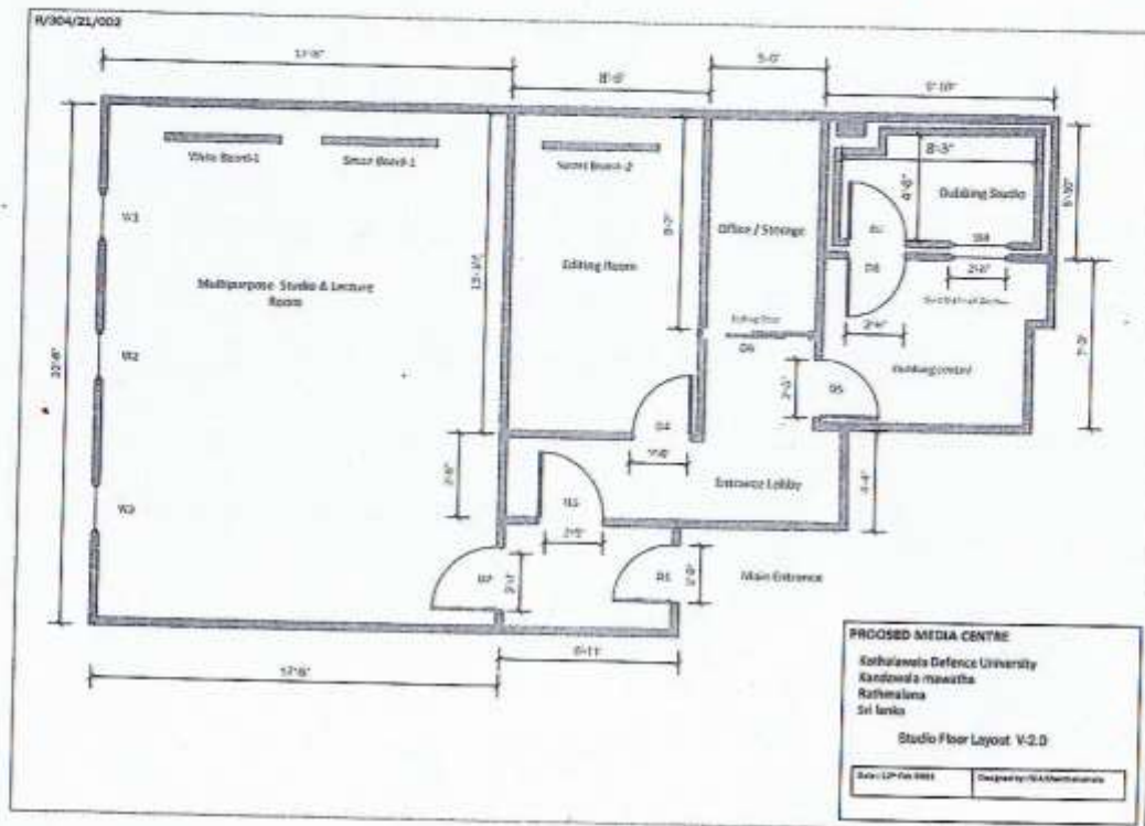
Diagram 2 : Partition layout with dimensions
