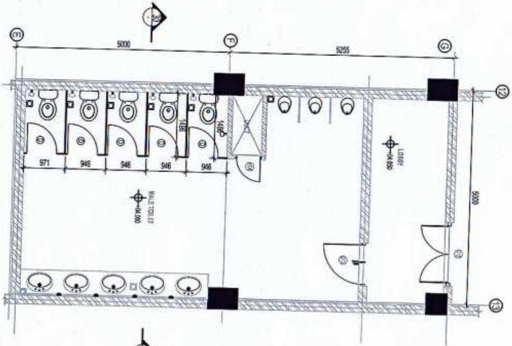
PLAN TOILET TYPE - T08 SCALE - 1:50 FIRST FLOOR
