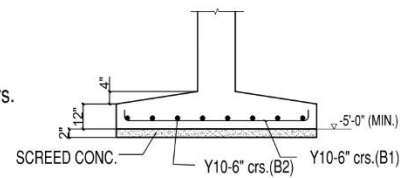
SECTION OF C1 & C2
