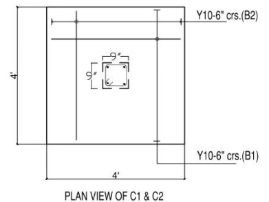
PLAN VIEW OF C1 & C2
