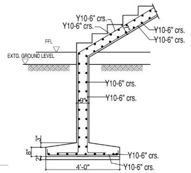
STAIRCASE FOUNDATION DETAIL
