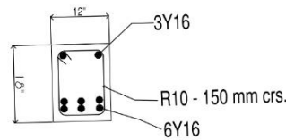
SECTION 3-3
