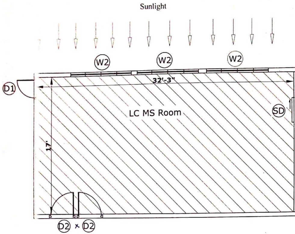
LAYOUT PLAN
