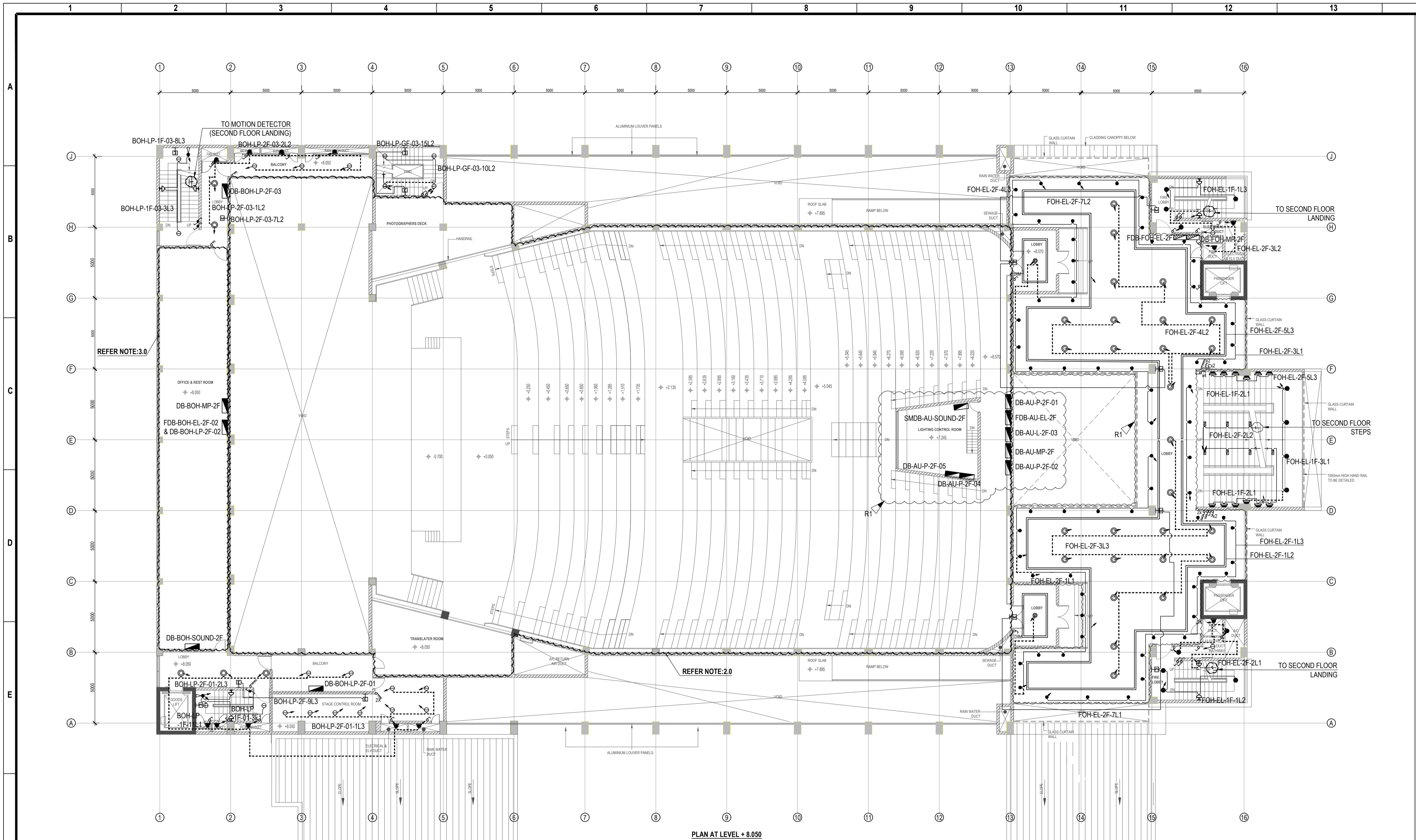
PLAN AT LEVEL +8.050
