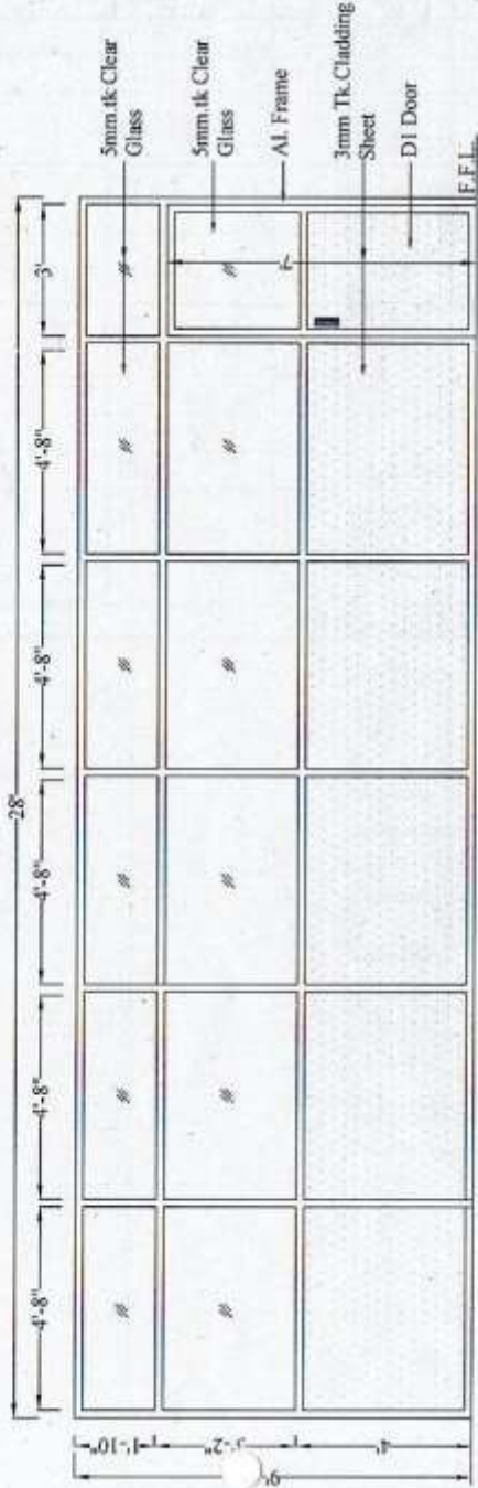
PARTITION 'A'
