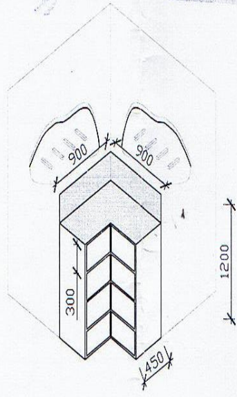
CP1- ISOMETRIC VIEW
